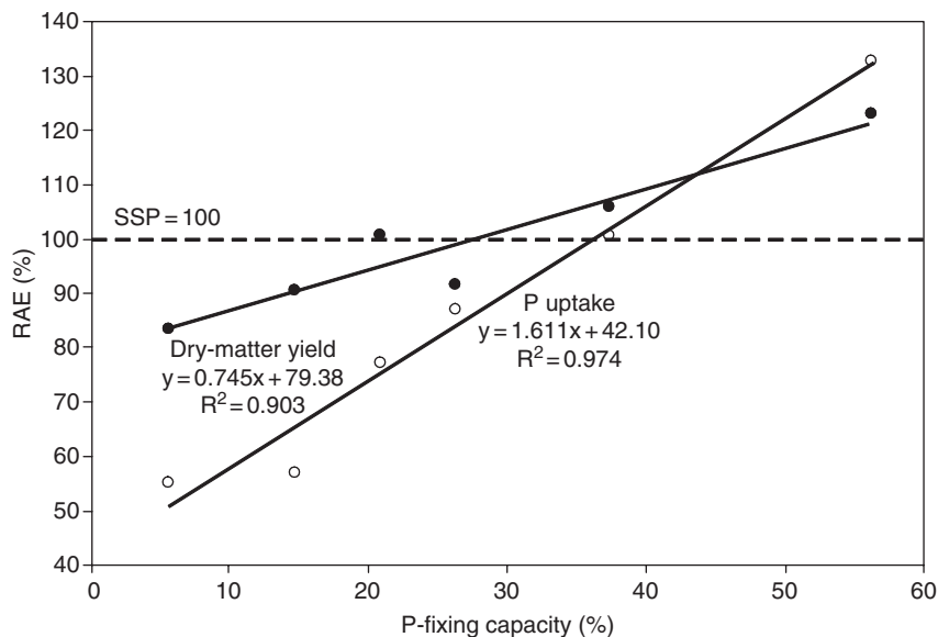
Figure 12 Relative agronomic effectiveness (RAE) in dry-matter yield and P uptake of maize obtained with PAPR-50% \text{H}_2\text{SO}_4 as related to soil P-fixing capacity. Source: Chien and Hammond (1989).
