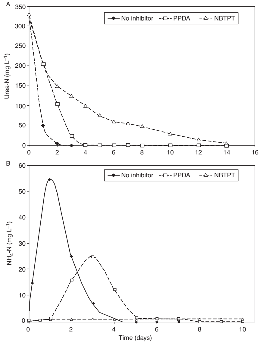
Figure 3 Concentrations of (A) urea-N and (B) NH 4 -N in floodwater treated with urea as affected by urease inhibitors. Source: Byrnes (1988).
