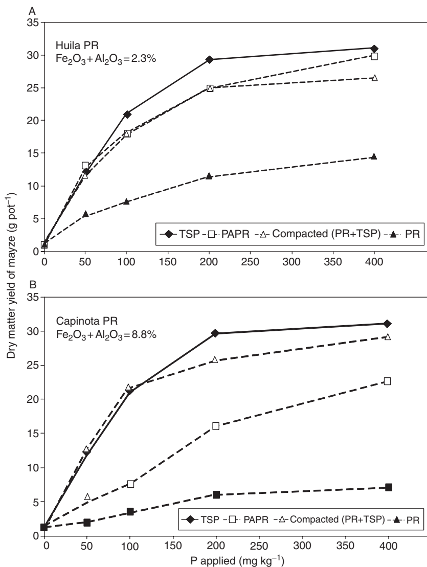
Figure 11 Dry-matter yield of maize obtained with TSP and modified PR products made from (A) Huila PR and (B) Capinota PR. Source: Menon and Chien (1990).
