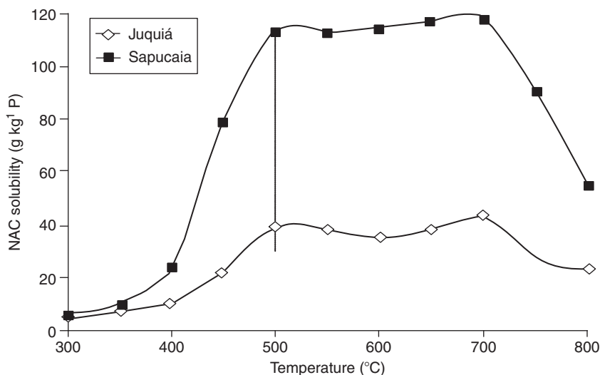
Figure 13 Effect of thermal treatment on neutral ammonium citrate (NAC) solubility of crandallite minerals from Juquía PR and Sapucaia PR deposits, Brazil. Source: Francisco et al. (2008b).
